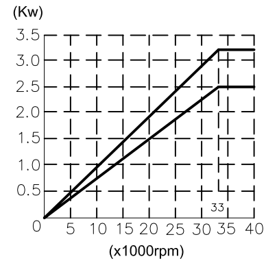
Power-diagram
