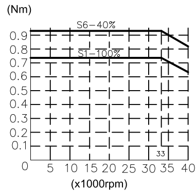
Torque-diagram
